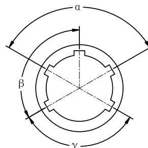
Plug front view
